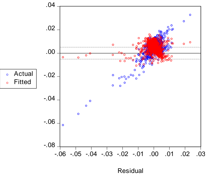
ROE model residuals plot against Y hat:
