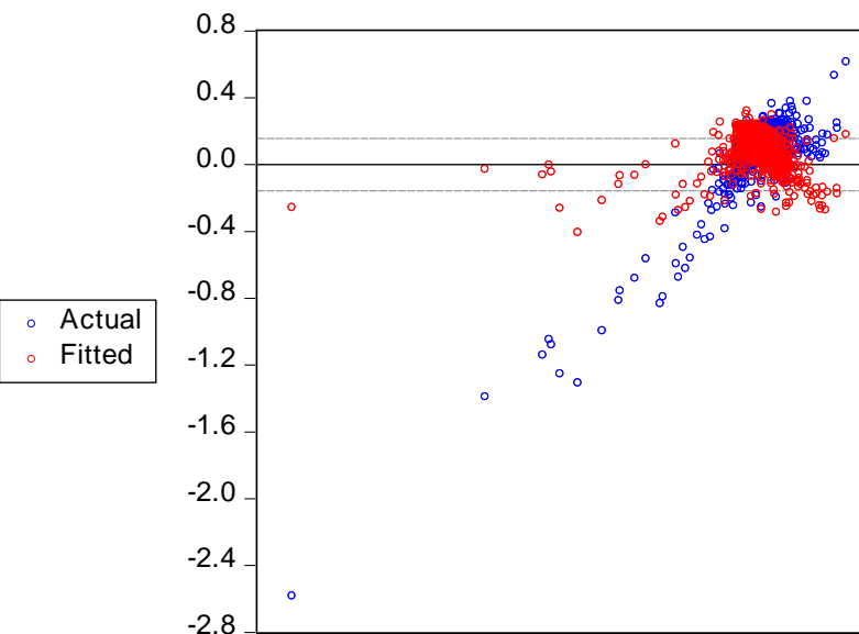
ROE model residuals plot against Y hat:
